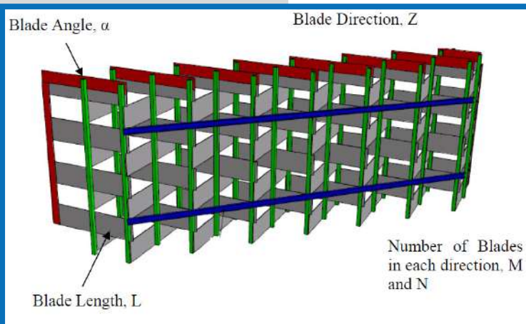
X-type static mixer, with design parameters
