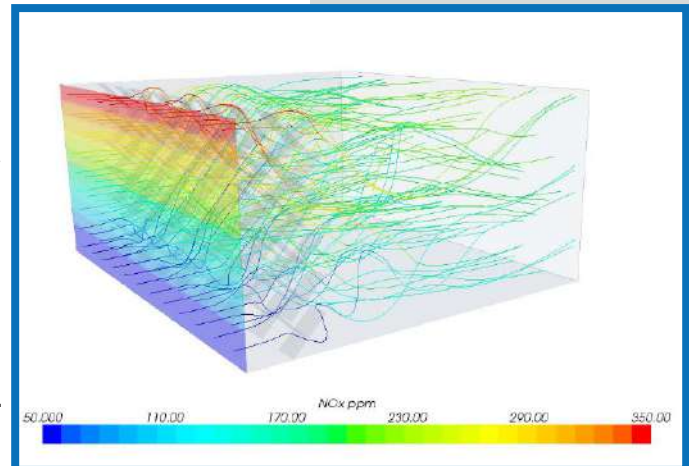
CFD Model of Static Mixer
