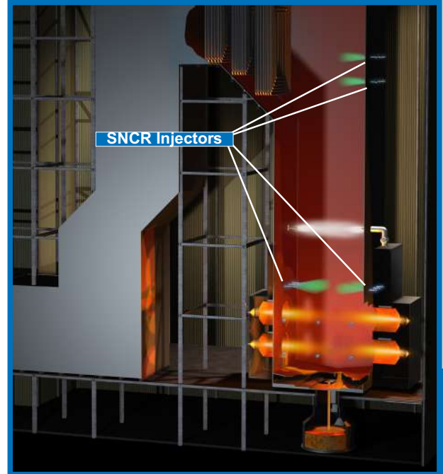
SNCR Injection Process
